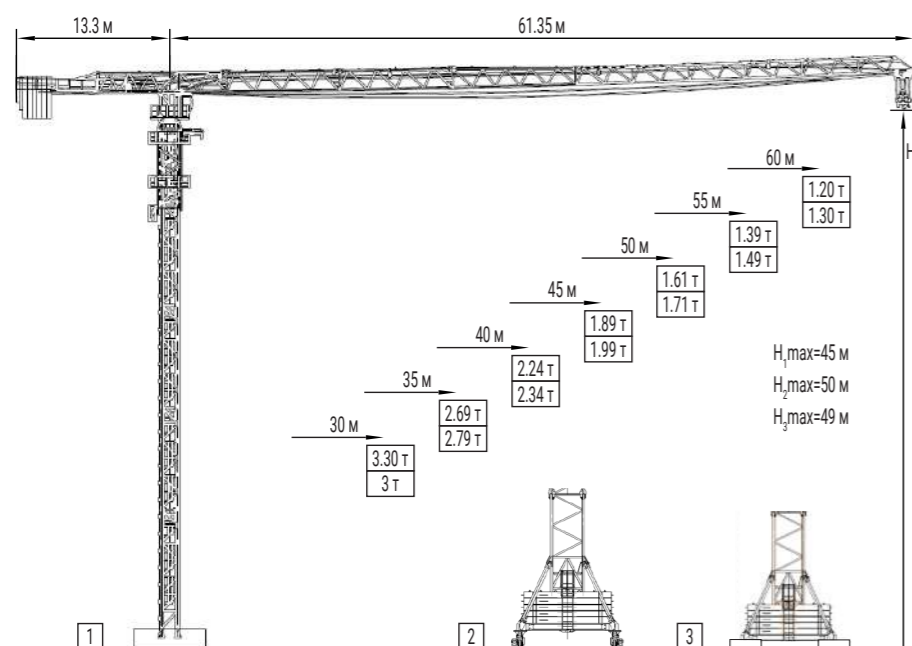
QTZ 100 (6013) – 6t
