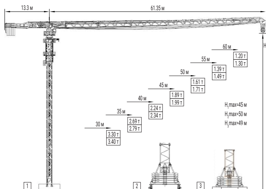
QTZ 100 (6013) – 8t
